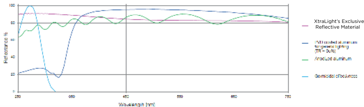
COMPARISON REFLECTANCE SPECTRA OF DIFFERENT MATERIALS
