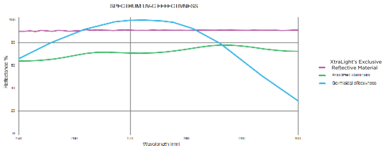
COMPARISON REFLECTANCE SPECTRA OF DIFFERENT MATERIALS
