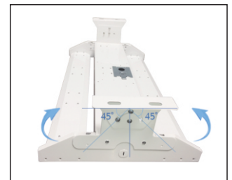
Surface Kit (45°adjustable angle)
