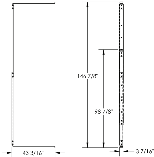
Adjustable Length to Fit Multiple Rack Measurements
