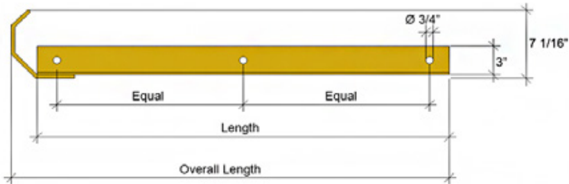
SINGLE SIDED WRAP AROUND LEFT CRESCENT - 42", 48", 54"
