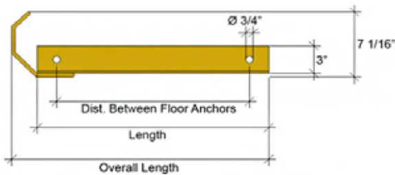
SINGLE SIDED WRAP AROUND LEFT CRESCENT - 24"
