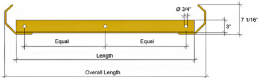
DOUBLE SIDED WRAP AROUND 42", 48"
